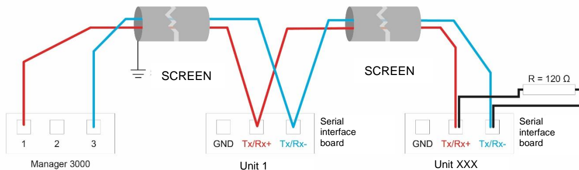
Figure 4-1: diagram showing a possible network layout with the Manager 3000.
