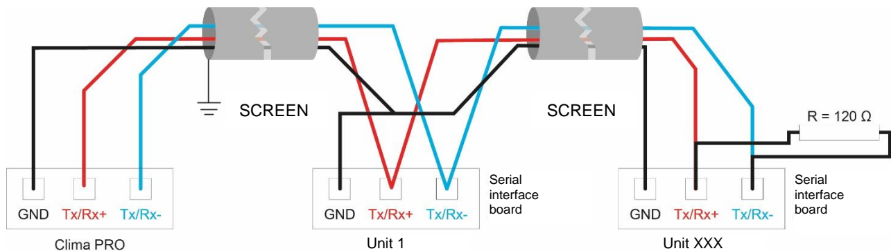
Figure 6-1: diagram showing a possible network layout with the ClimaPRO.
