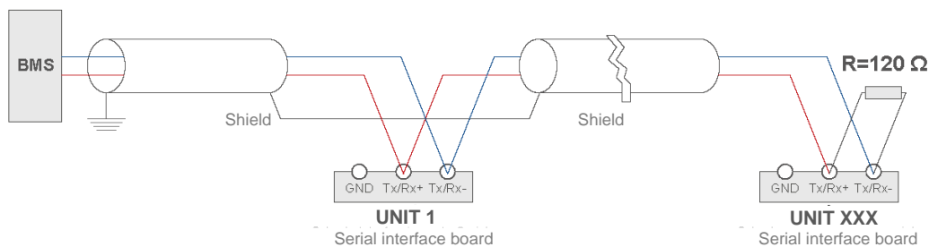
Figure 17-1: summary diagram showing a possible BMS supervision network layout.
