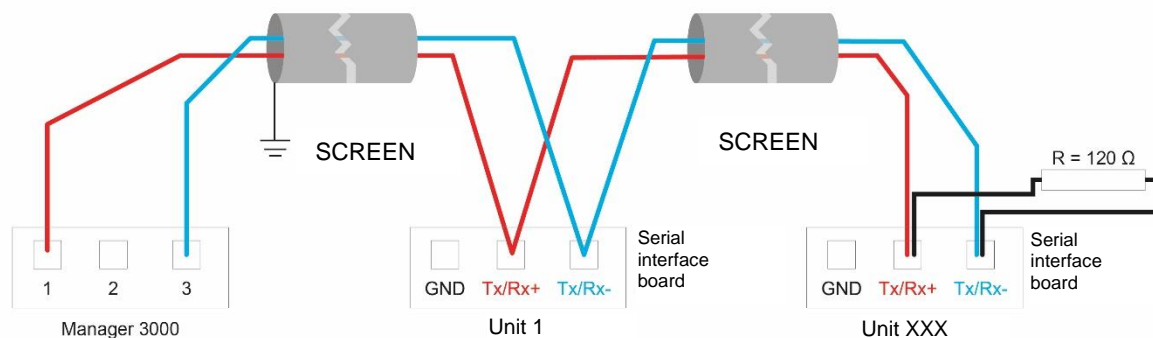
Figure 5-1: diagram showing a possible network layout with the Manager 3000+.
