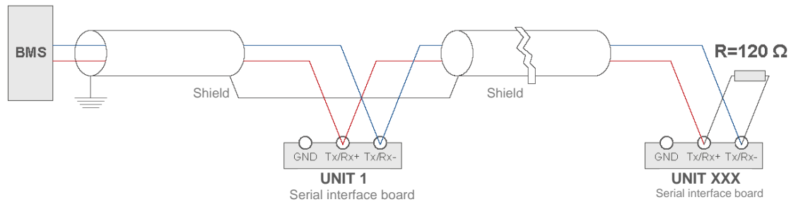
Figure 8-1: summary diagram showing a possible BMS supervision network layout.
