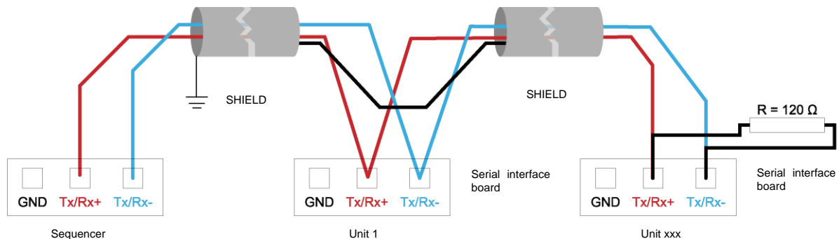
Figure 3-1: diagram showing a possible network layout with the Sequencer.
